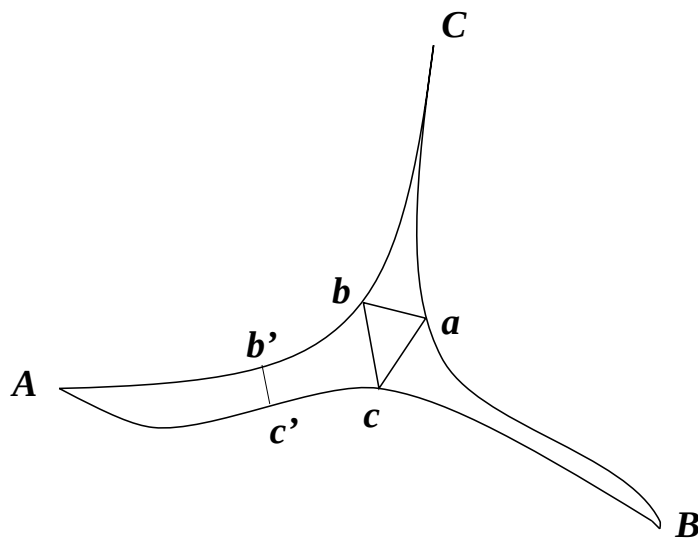
FIGURE 1. Thin triangle
